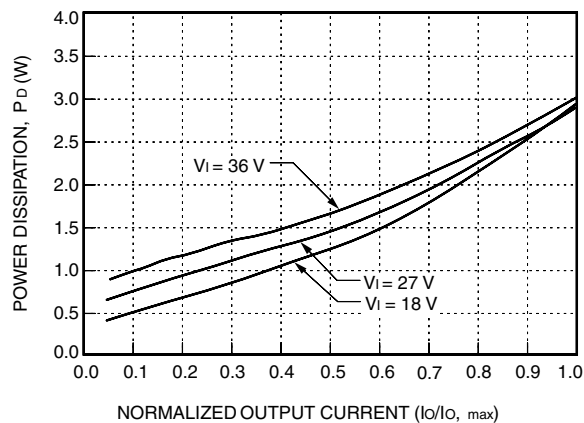
Figure 50. LC010A, B, C Typical Power Dissipation vs. Normalized Output Current at Tc = 25 °C
